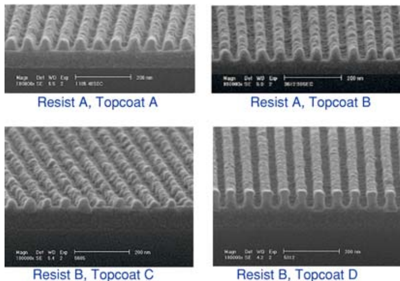
Fig. 21 32-nm imagery using ASML interference immersion test rig with DuPont IF-132 immersion fluid for a matrix of resists and topcoats.
