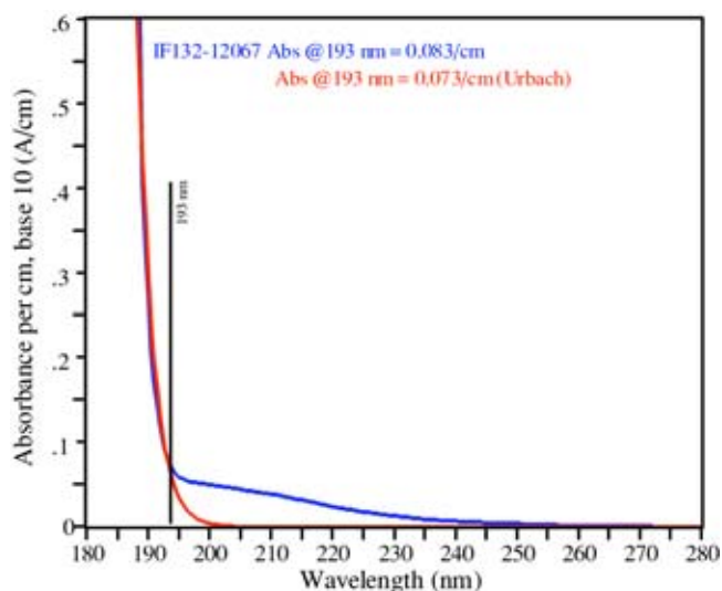
Fig. 17 Optical absorption edge and Urbach edge for IF132 showing a low absorbance second-generation immersion fluid.
