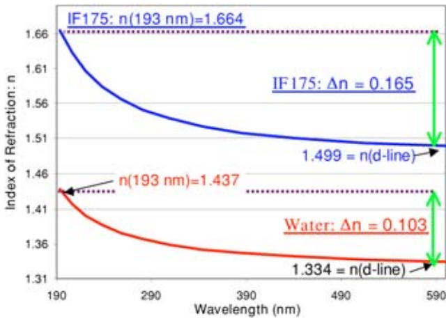
Fig. 18 Spectral refractive index of IF175 compared to the refractive index of water. Note IF175's increased n_d , dispersion \Delta n , and n_{193} .
