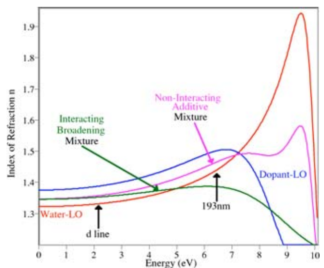
Fig. 16 Lorentz oscillator models, representing 50:50 mixtures of water and a TEOS-like dopant, based on two approaches: a noninteracting (additive) mixture and an interacting (broadening) mixture. Note the changes in the n_d and n_{193} , and the dispersion for the two different models.
