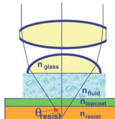
Fig. 8 Immersion lithography film stack.
