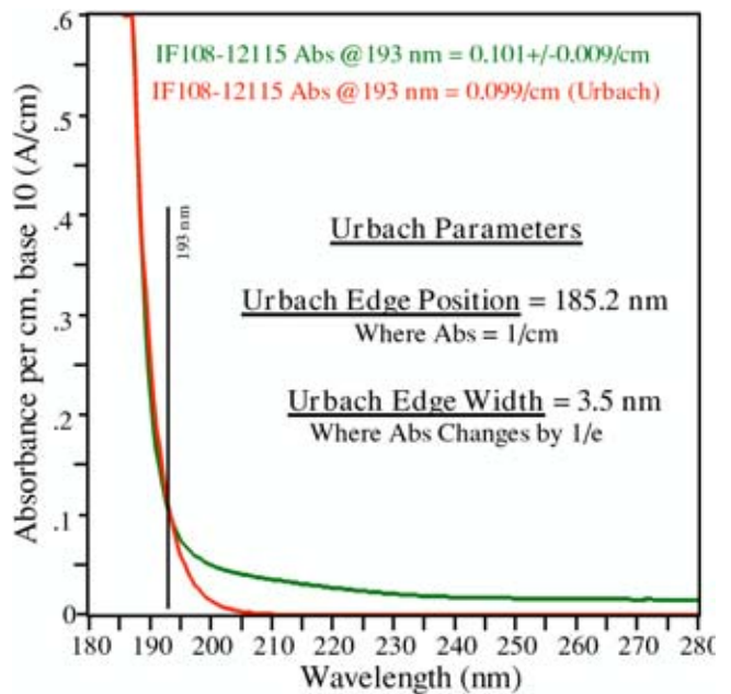
Fig. 12 Optical absorbance of 17.6-megohm water, measured using relative transmission measurement at three thicknesses. The Urbach edge fit to this absorption edge is also shown along with the Urbach fit parameters.
