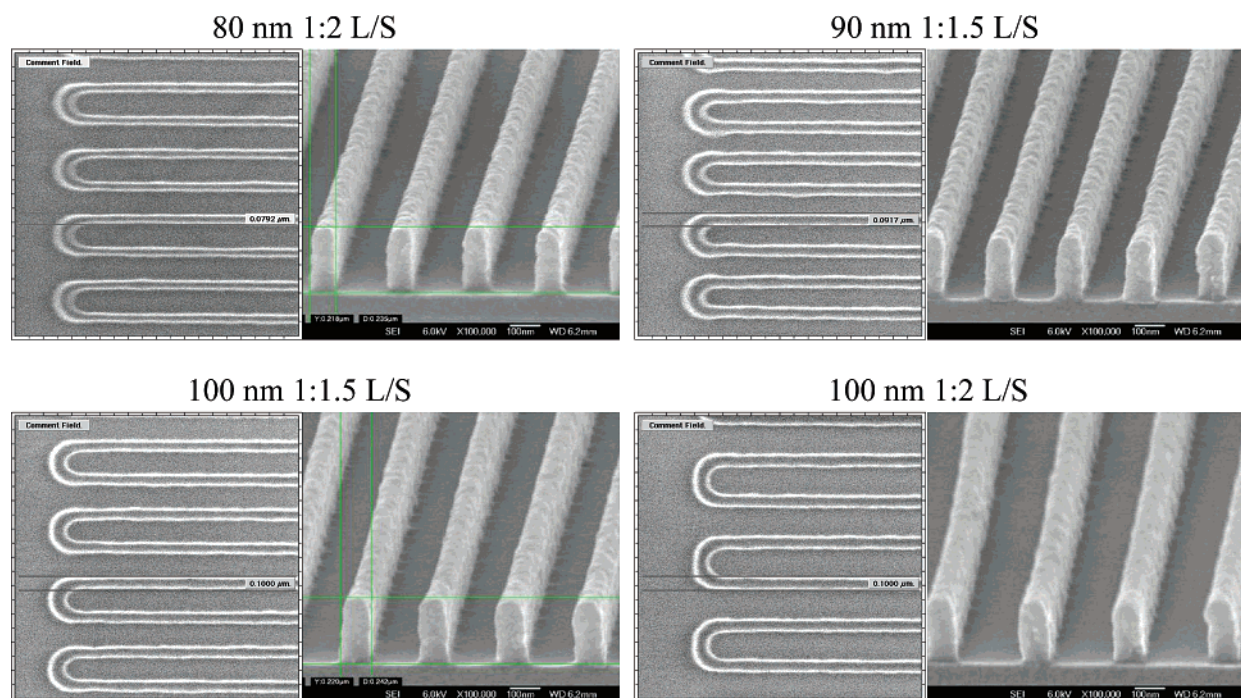
Figure 13. SEM pictures of a tetrapolymer 28 demonstrating dense and semidense lines.
