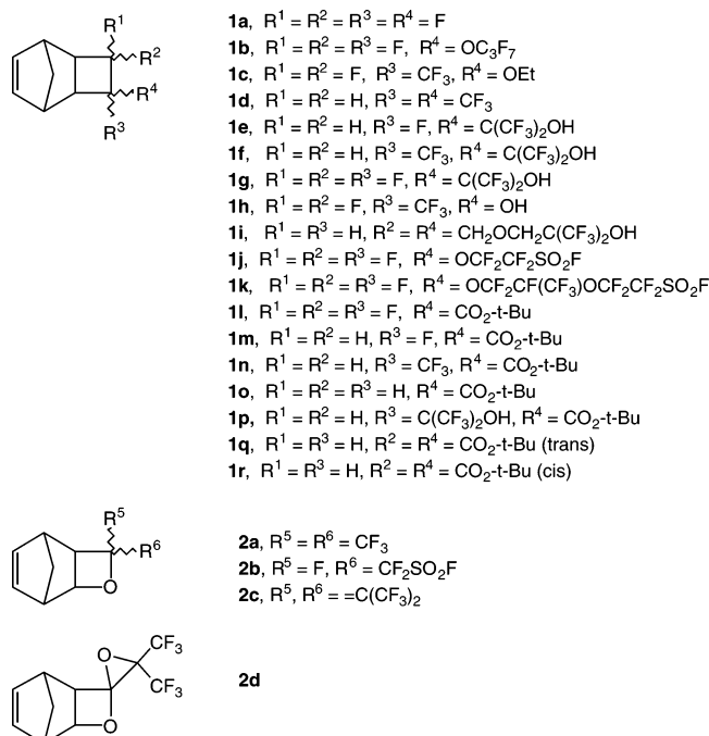
Figure 3. Tricyclonene (TCN) monomers.
