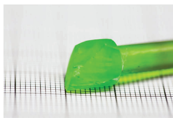
\text{NaCaNi}_2\text{F}_7
