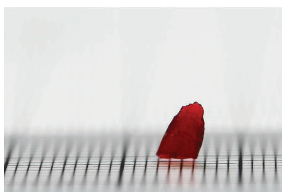
\text{NaCaCo}_2\text{F}_7
